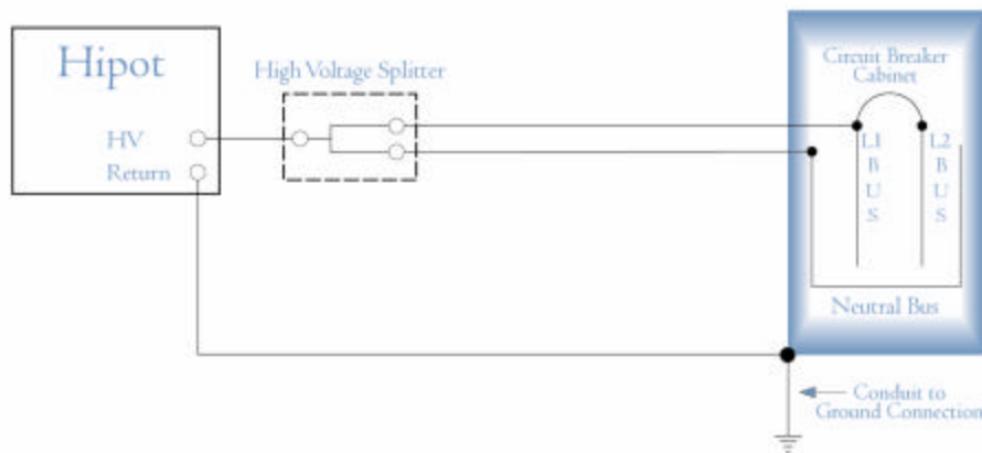
Figure 3 Hipot Tests of Manufactured and Modular Homes
