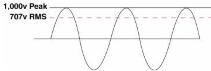
Figure 1 RMS Voltages vs. Peak Voltages
