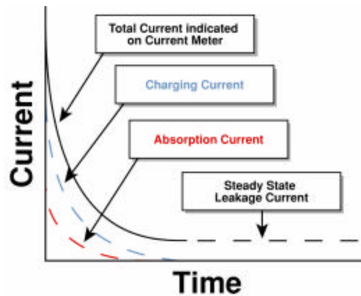
Figure 2 Direct Current vs. Time
